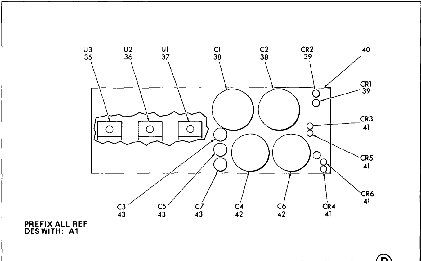
Figure 2. Chassis Assembly, P1122-014-02 (Sheet 2 of 2)
