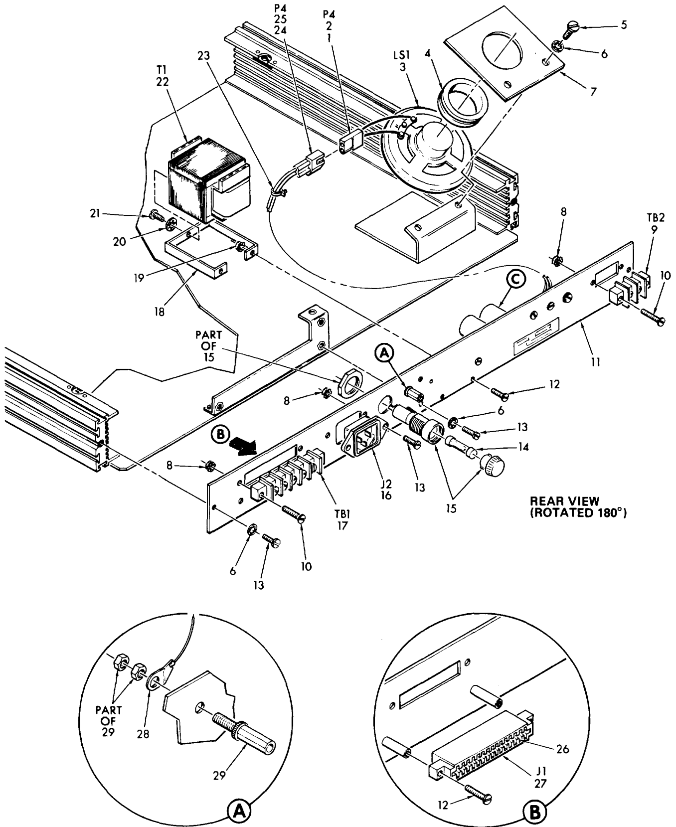
Figure 2. Chassis Assembly, P1122-014-02 (Sheet 1 of 2)
