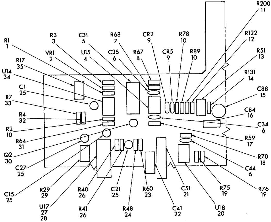
Figure 4. Circuit Card Assembly, P1122-003-02 (Sheet 1 of 10)
