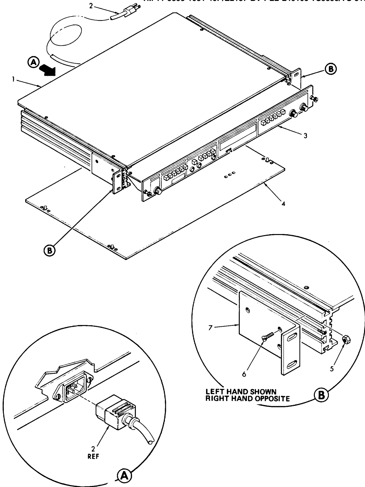
Figure 1. Test Set, Telephone, TS-3853-G
