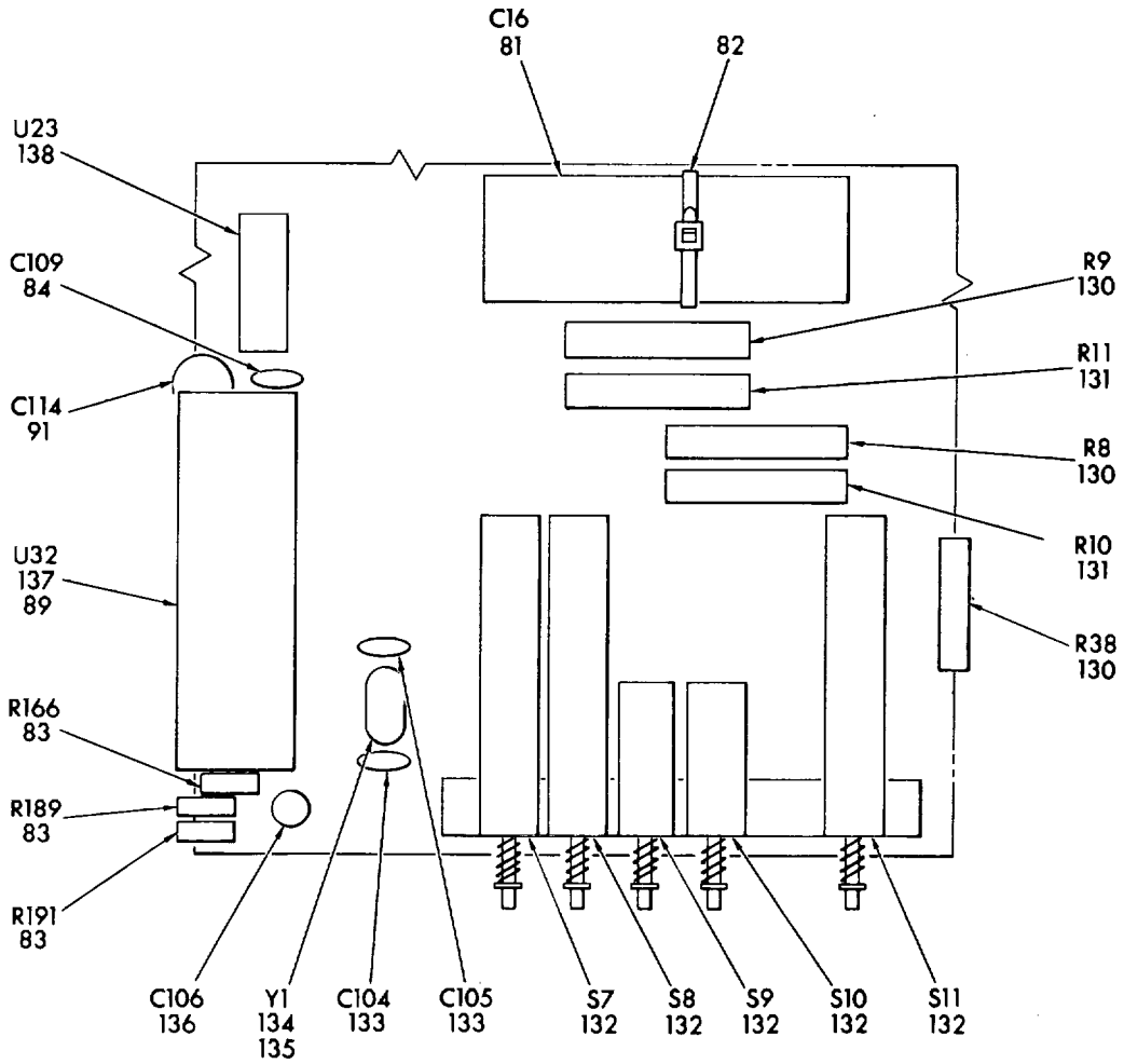
Figure 4. Circuit Card Assembly, P1122-003-02 (Sheet 7 of 10)
