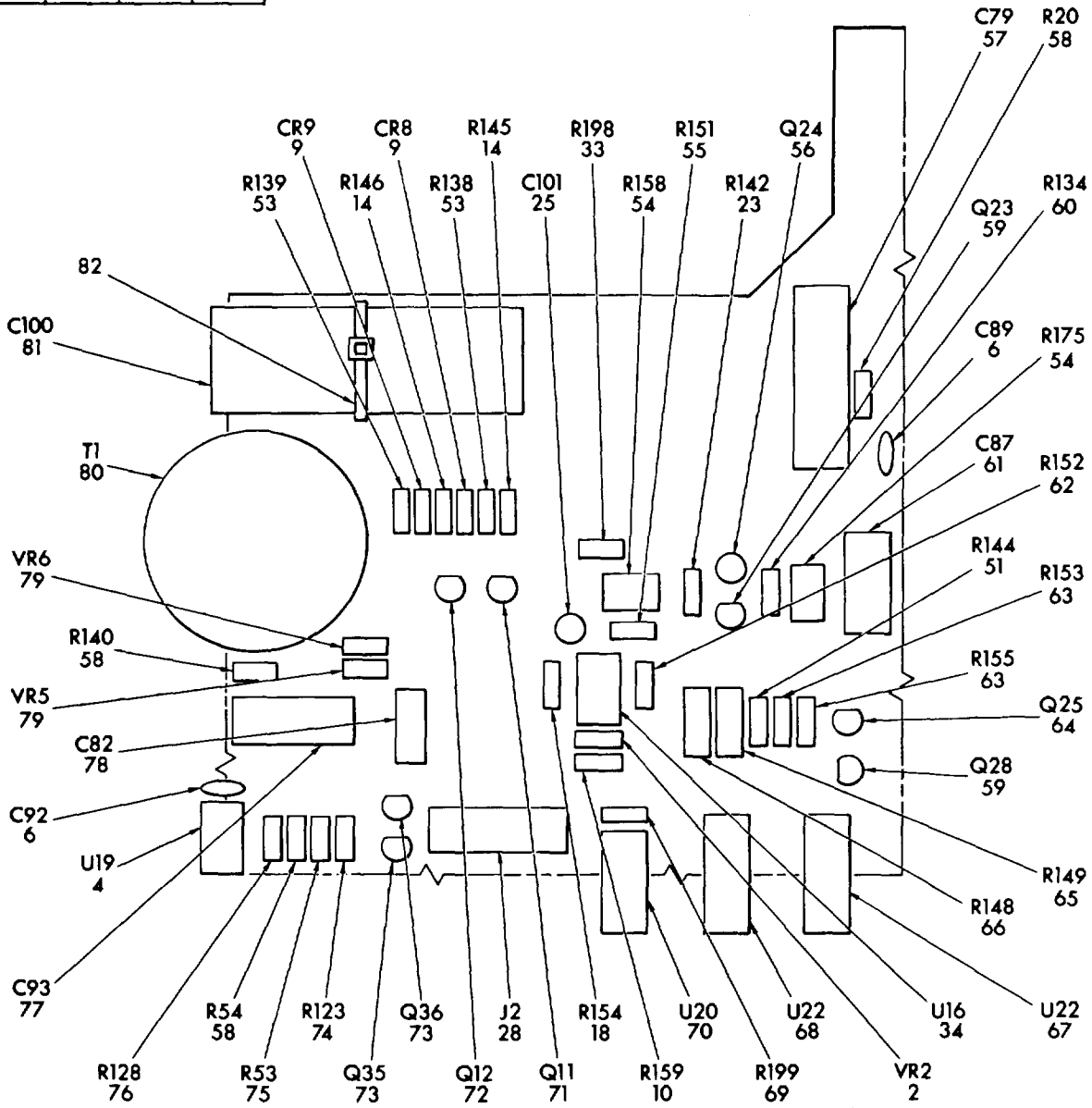
Figure 4. Circuit Card Assembly, P1122-003-02 (Sheet 3 of 10)
