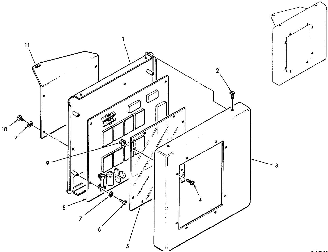
Figure 5. Indicator, Digital Display, ID-2233/U
