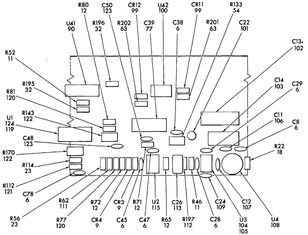
Figure 4. Circuit Card Assembly, P1122-003-02 (Sheet 5 of 10)
