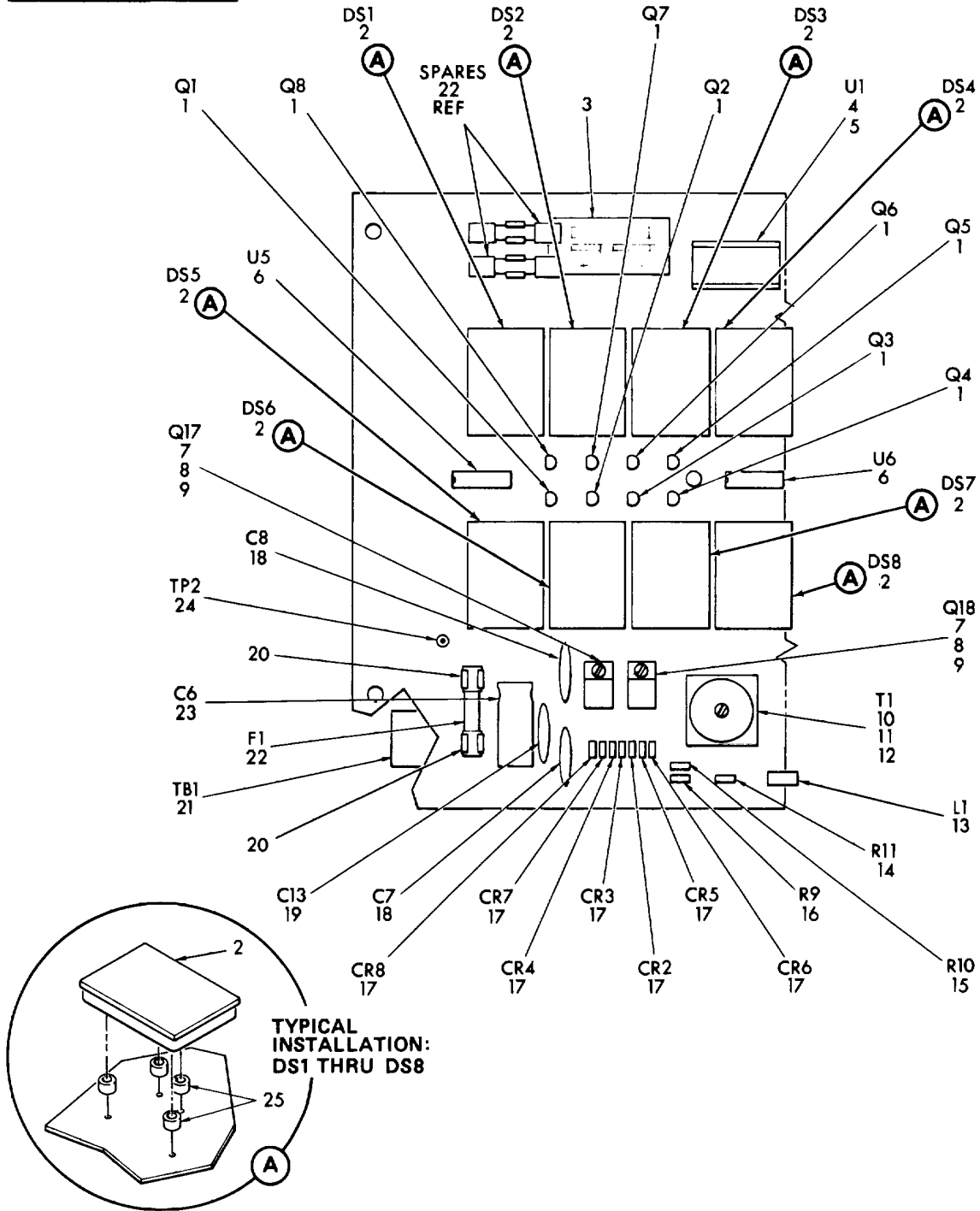
Figure 6. Circuit Card Assembly, P1122-022-01 (Sheet 1 of 2)
