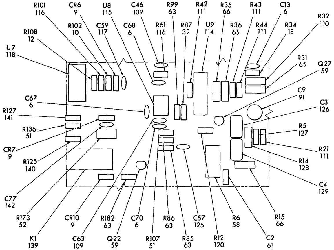
Figure 4. Circuit Card Assembly, P1122-003-02 Sheet 6 of 10)
